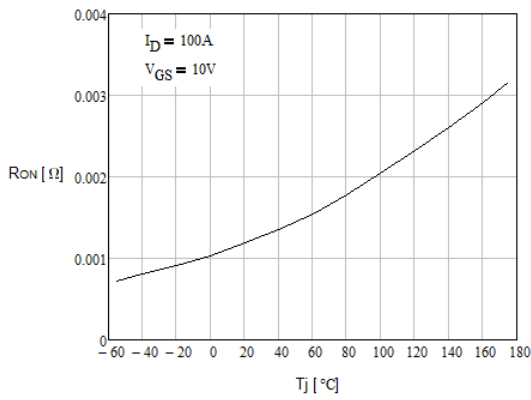
Typical Ron vs. Temp
