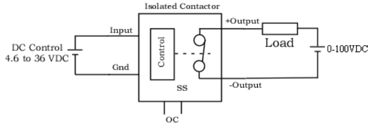
DC Supply
