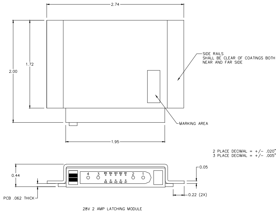
Figure 7: SRPC7D28 Mechanical Dimensions / Connector Keying
