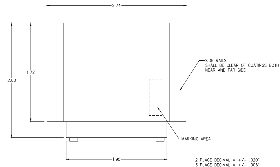
Figure 9: SRPC15D28 Mechanical Dimensions / Connector Keying
