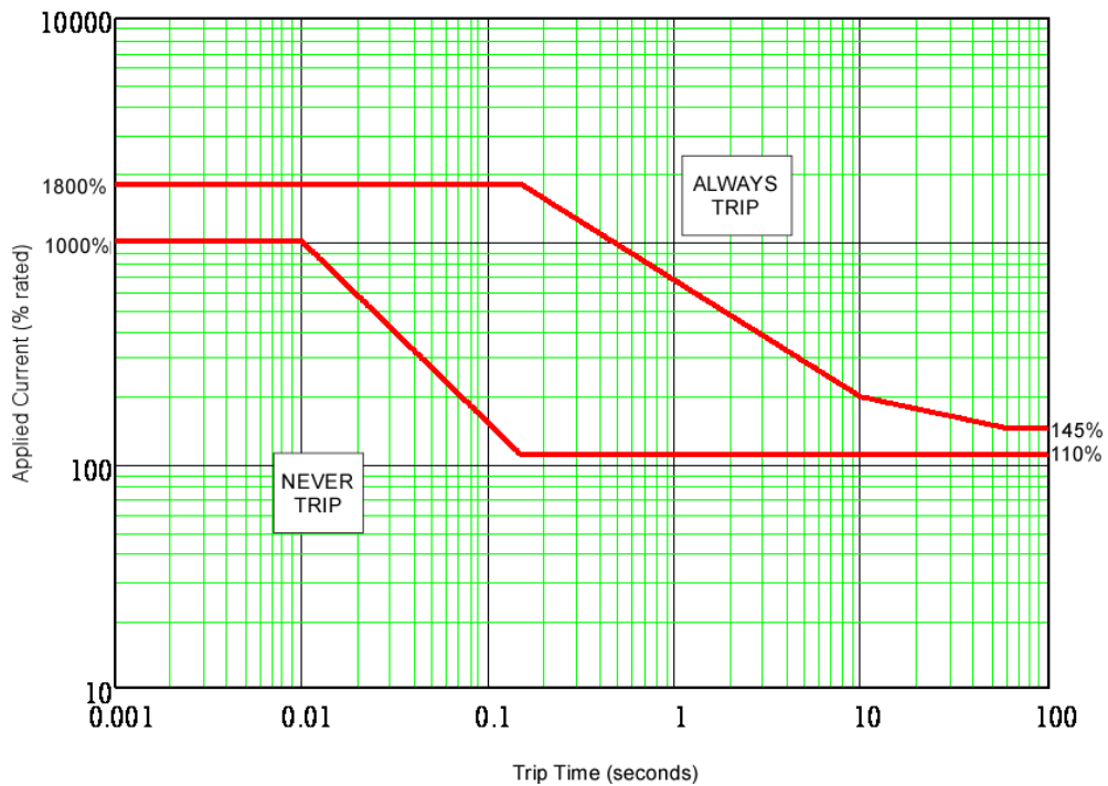
Figure 2: Trip Curve for SRPC7D28 and SRPC7D28F
