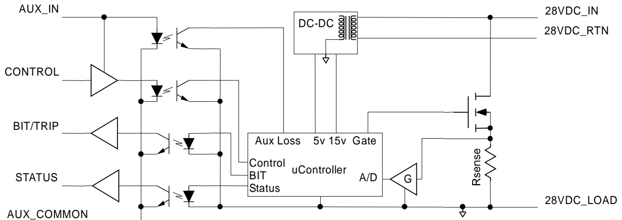
Figure 11: Electrical Block Diagram
