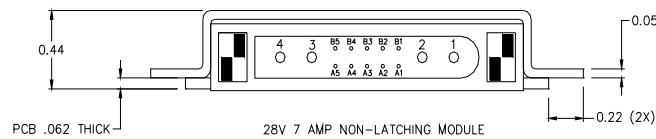
Figure 9: SRPC15D28 Mechanical Dimensions / Connector Keying
