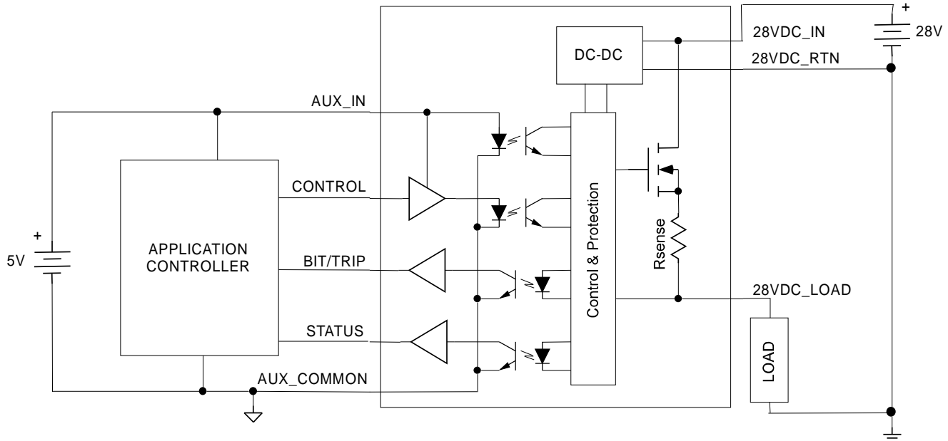
Figure 12: Typical Application
