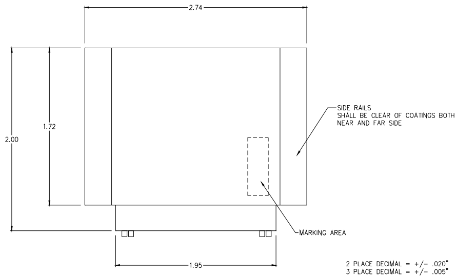
Figure 8: SRPC7D28F Mechanical Dimensions / Connector Keying
