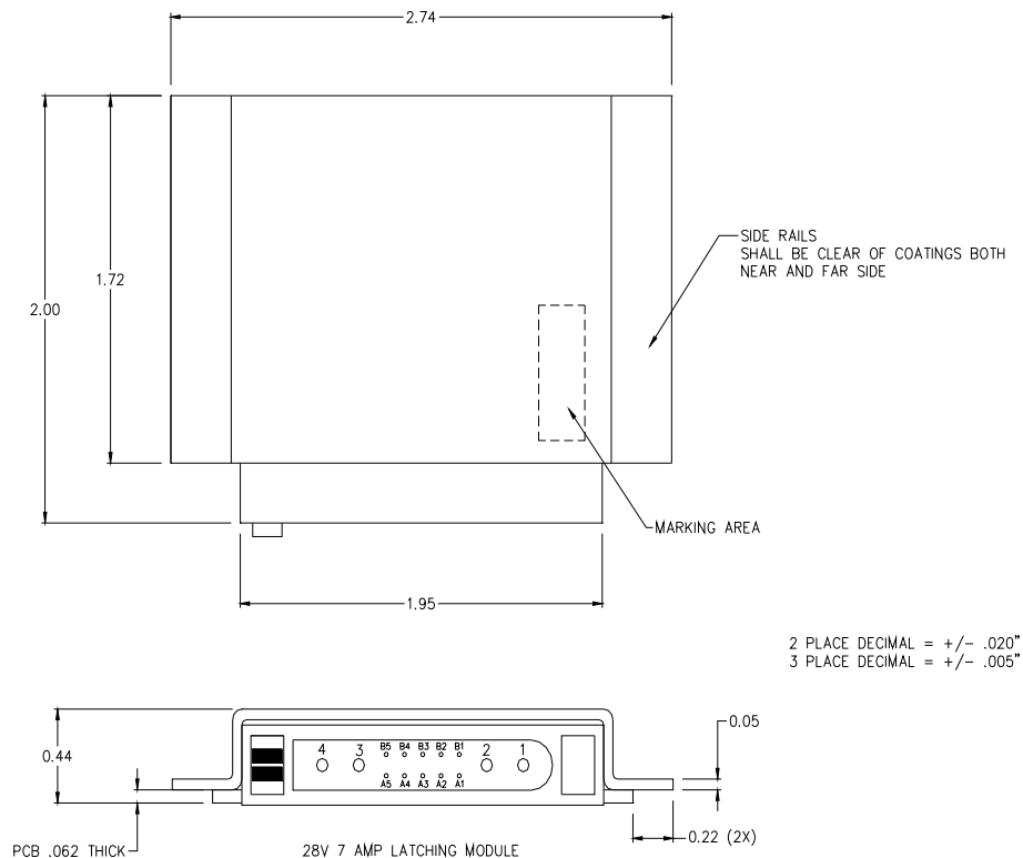
Figure 7: SRPC7D28 Mechanical Dimensions / Connector Keying
