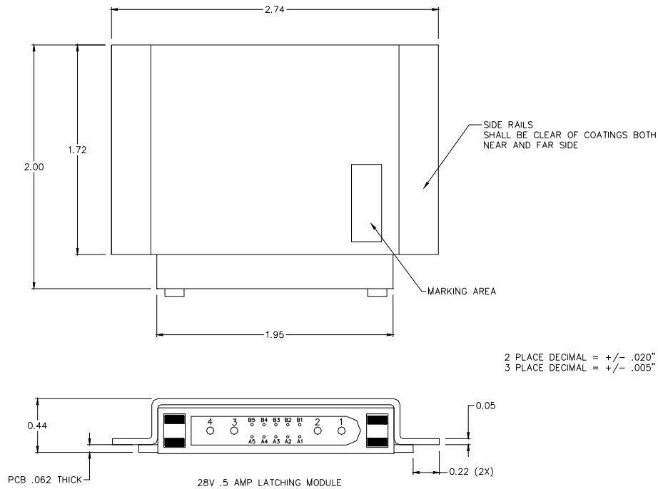
Figure 5: SRPC0.5D28 Mechanical Dimensions / Connector Keying
