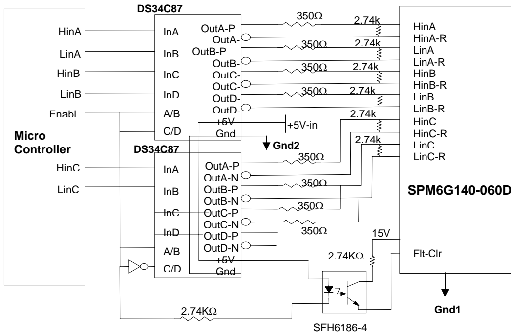
Fig. 9 Input Interface and Startup Circuit
